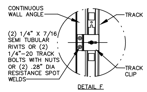
DETAIL F
